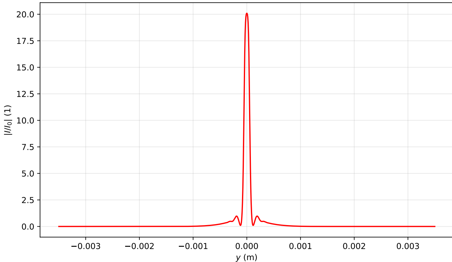
Intensity profile I(x=0, y, z=0.478)/I_0 , P_{in}=5.5P_{cr} , artificial time
